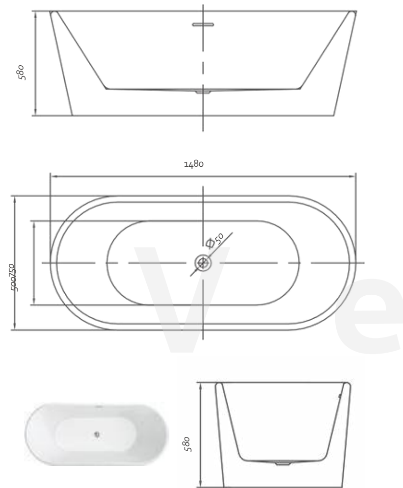
VBM-YQ5001S-15 Size: 1480x750x580mm
